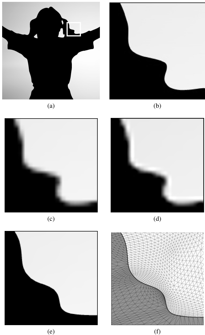
Fig. 3: Scaling results obtained by the bilinear, bicubic, and proposed methods for backlight image with \alpha = 8 . (a) The high-resolution image with region of interest marked with white rectangle. The same region obtained from the (b) high-resolution image, (c) bilinear (PEE 55.17), (d) bicubic (PEE 47.58), and (e) proposed methods (PEE 0.95). (f) The subdivided mesh corresponding to the result shown in (e), with the constrained edges shown as thick lines.
