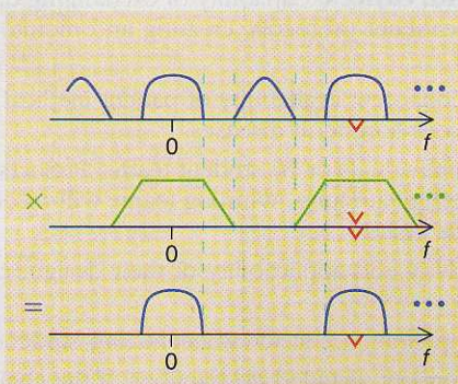
Fig. 5 A digital filter applies a periodic frequency response to a discrete-time input.
