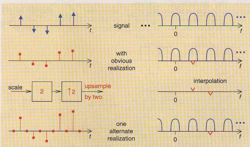
Fig. 2 Interpolation leaves the signal unchanged but transforms its realization to a higher sample rate.
