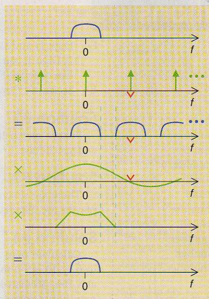
Fig. 4 Sampling and reconstruction of the signal sampled.
