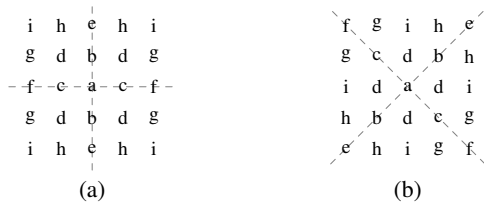
Fig. 3. Types of four-fold symmetry. (a) Quadrantal centrosymmetry and (b) rotated quadrantal centrosymmetry.
