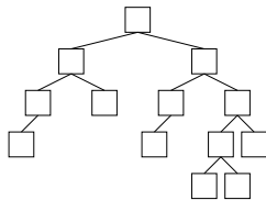
Height Balanced
