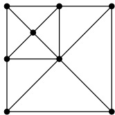
Delaunay Triangulation
