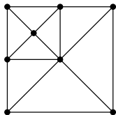
Triangulation
