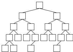
Strictly Balanced
