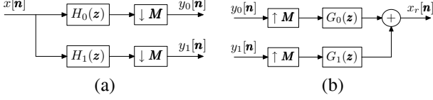
FIGURE 1: The canonical form of a quincunx filter bank. (a) Analysis side and (b) synthesis side.
