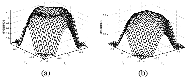
FIGURE 8: Frequency responses of the (a) lowpass analysis and (b) lowpass synthesis filters of OPT3.
