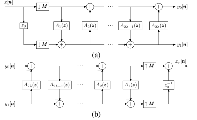
FIGURE 4: Lifting realization of a quincunx filter bank. (a) Analysis side and (b) synthesis side.
