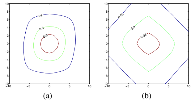
FIGURE 13: The contour plots of the autocorrelation functions of the (a) sar2 and (b) gold images.
