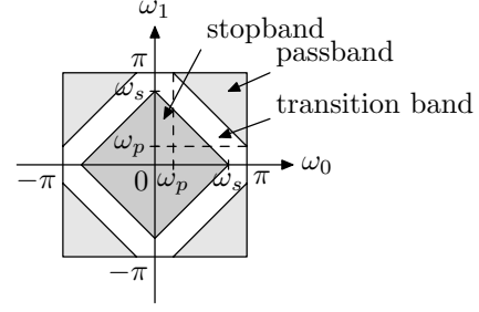
FIGURE 6: Weighting function for a highpass filter with diamond-shaped stopband.
