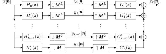
FIGURE 3: The equivalent nonuniform filter bank associated with the L -level octave-band filter bank.
