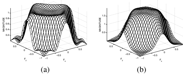
FIGURE 7: Frequency responses of the (a) lowpass analysis and (b) lowpass synthesis filters of OPT1.
