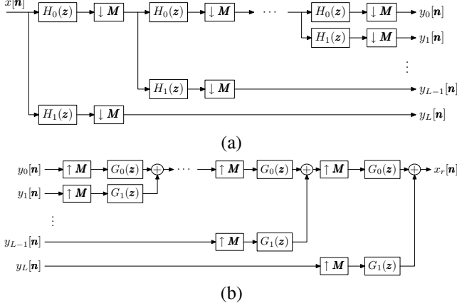
FIGURE 2: The structure of an L -level octave-band filter bank. (a) Analysis side and (b) synthesis side.
