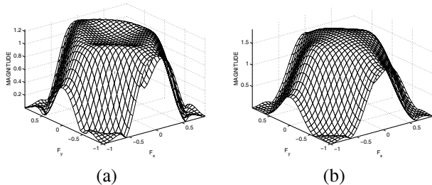
FIGURE 9: Frequency responses of the (a) lowpass analysis and (b) lowpass synthesis filters of OPT4.
