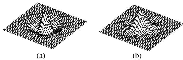
FIGURE 11: The (a) primal wavelet and (b) primal scaling functions for OPT3.
