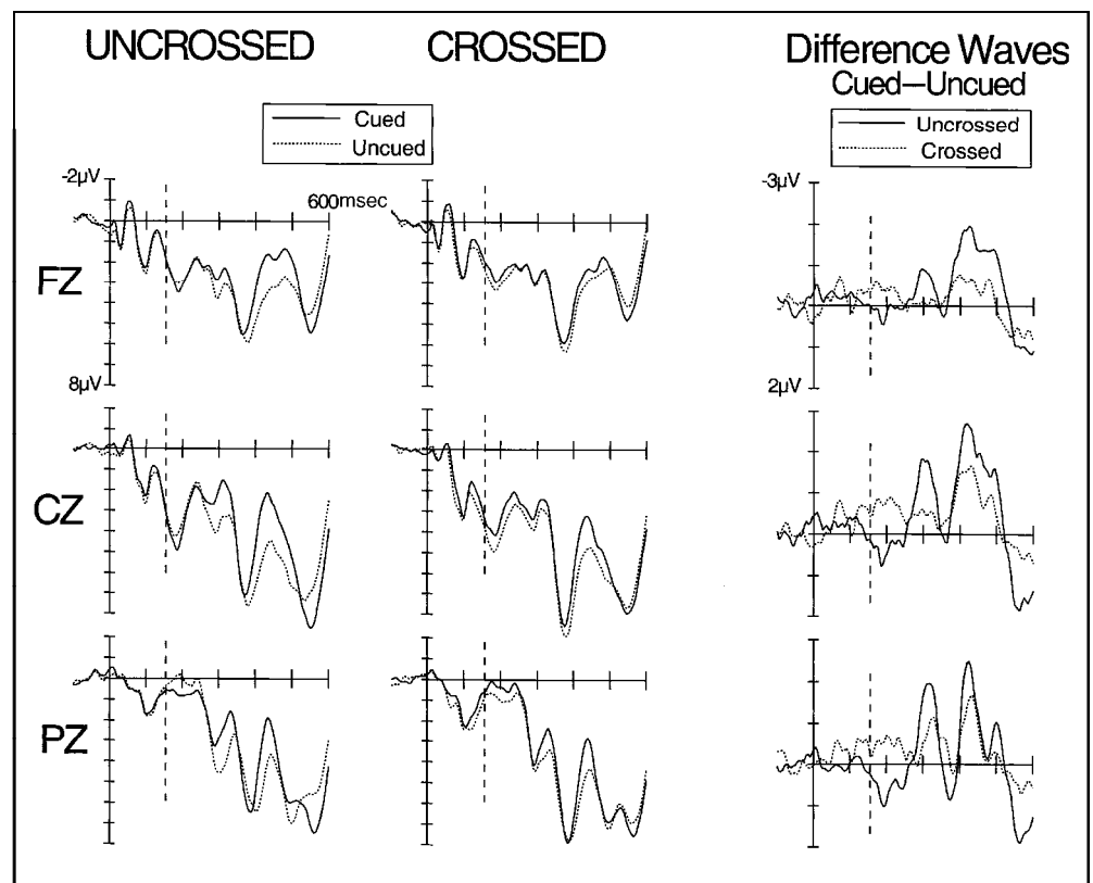
Figure 4. Left: Grand-averaged ERPs, collapsed across visual stimulus side, obtained at Fz, Cz, and Pz in short -SOA blocks for cued (solid curve) and uncued (dotted curve) trials, displayed separately for uncrossed hands (left) and crossed hands (middle). Right: Difference waveforms obtained at midline electrodes by subtracting ERPs for uncued trials from ERPs for cued trials for uncrossed-hand blocks (solid lines) and crossed-hand blocks (dotted lines). All waveforms are plotted with y -axes at the onset of the tactile cue and dashed vertical lines marking the onset of visual stimulus.
