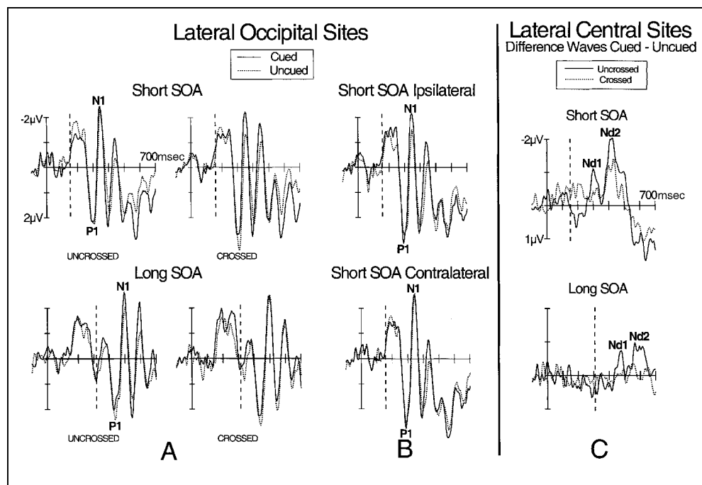
Figure 3. (A) Grand-averaged ERPs collapsed across right and left occipital electrodes and visual stimulus positions for cued (solid curves) and uncued (dotted curves) trials for the four conditions (2 SOAs \times 2 Hand Postures). (B) Grand-averaged ERPs at the short SOA for occipital electrodes ipsilateral (top) and contralateral (bottom) to the visual stimulus, collapsed across hand position. (C) Difference waveforms obtained by subtracting ERPs for uncued trials from ERPs for cued trials, summed across lateral central sites for uncrossed (solid curves) and crossed (dotted curves) hand posture, and plotted separately for long versus short SOAs. All waveforms are plotted with y-axes at the onset of the tactile cue and dashed vertical lines marking the onset of visual stimulus.
