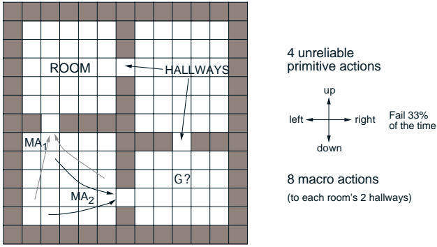
Figure 1: Example Task. The natural macro actions are to move from room to room.
