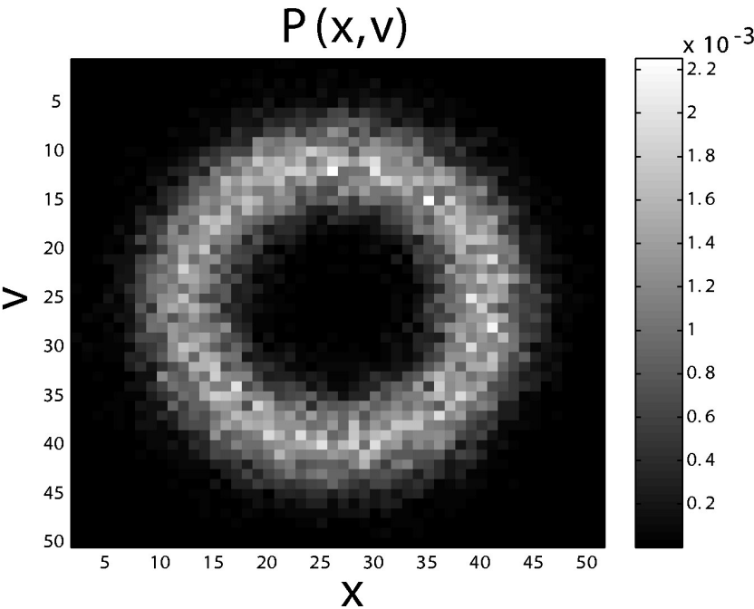
Figure 7: Twenty thousand data points drawn from a radial distribution, according to P(r) = \mathcal{N}(1, 0.2) , with x = r\cos(\phi) , v = r\sin(\phi) , and P(\phi) = 1/2\pi . Displayed is the estimated probability distribution (normalized histogram with 50 bins along each axis).
