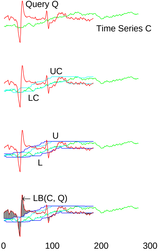
Figure 4: An illustration of the SWM envelopes. From top to bottom: A time series C and a query Q ; The series C bounded from above and below respectively by UC and LC , the envelope for scaling; The series UC bounded above by U and LC bounded below by L , forming the overall envelope for scaling and time warping; and the lower bounding distance LB derived from the overall envelope.
