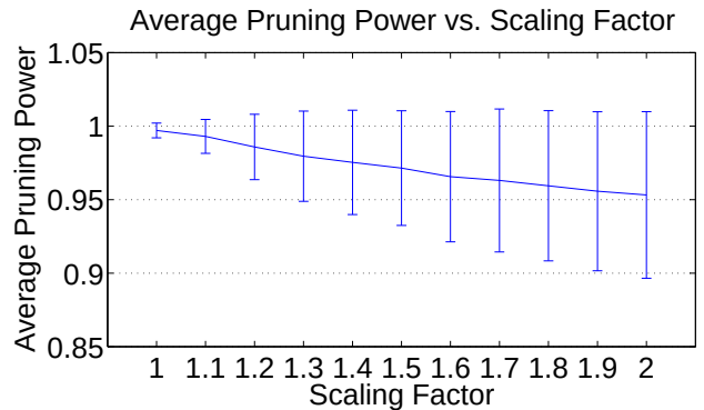
Figure 16: Average pruning power vs. scaling factor
