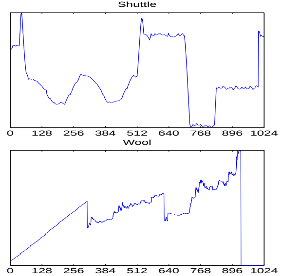
Figure 14: Data giving the lowest pruning power
