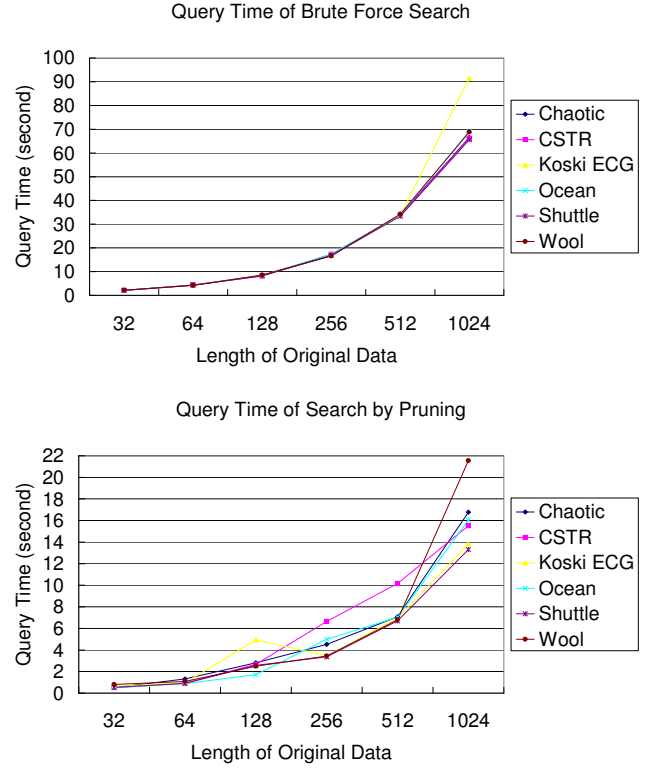
Figure 12: Query time comparison
