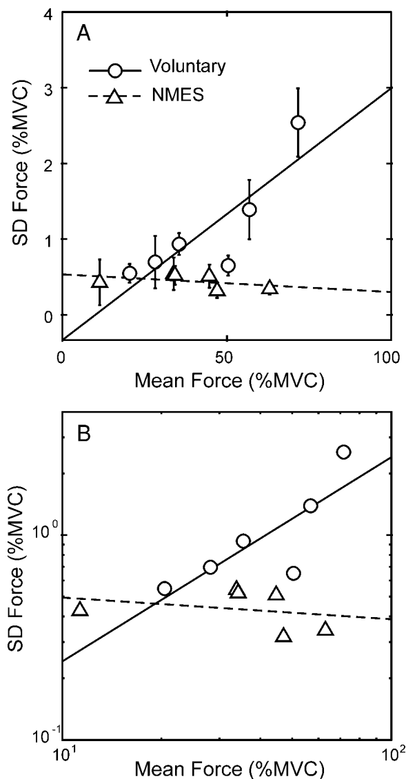
FIG. 2. The scaling of force variability with respect to mean force output. A: data from subject 1 is shown. The SD of the force output is positively correlated to the mean force only in the voluntary condition. B: same data as above, plotted on a log-log scale with regression lines to determine whether the signal-dependent noise (SDN) exhibits linear scaling, i.e., slope = 1.0. Slope in the voluntary condition is 0.99 and in the NMES condition is -0.10 , but the latter was not significant.
