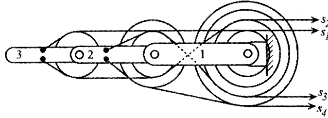
Figure 1. Planar scheme of Stanford/JPL manipulator, a typical 3-links tendon mechanism, with 4 independent transmission chains s_1 \dots s_4 .
