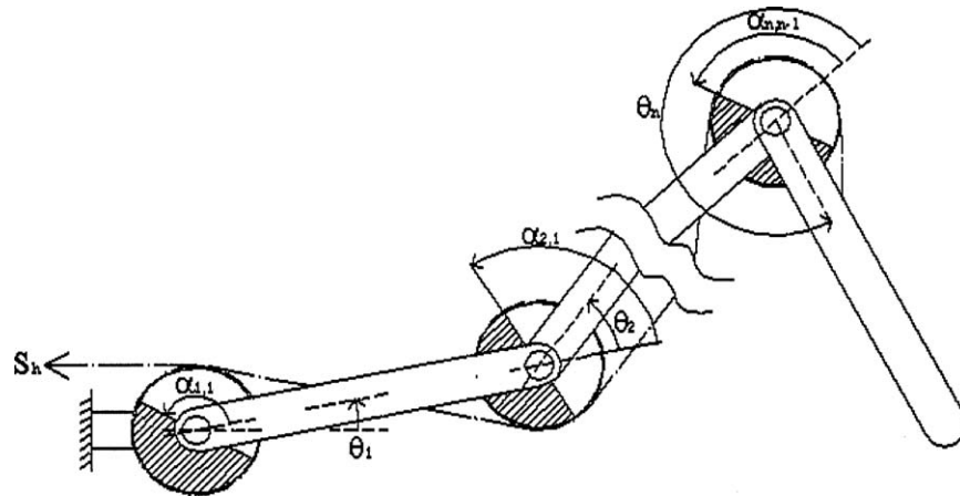
Figure 3. Nomenclature of the transmission chain.
