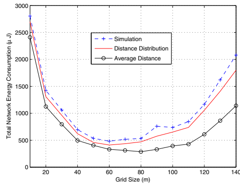
Fig. 8. Total Network Energy Consumption with Diagonal-First Routing.
