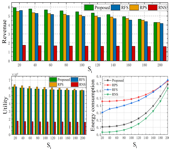
Fig. 10: Revenue, utility and vehicular energy consumption in data trading with different data sizes.
