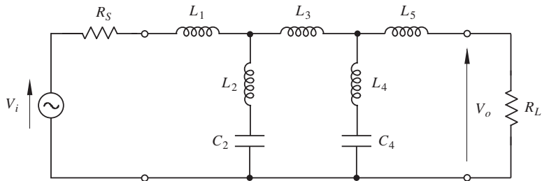
Passive RLC lowpass filter
