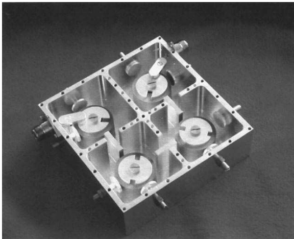
Microwave bandpass filter
