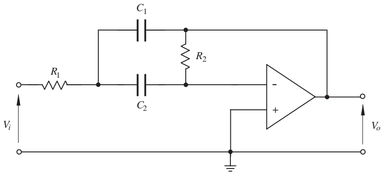
Discrete active bandpass filter
