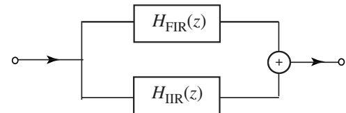
Fig. 1. Structure of a composite filter.
