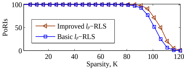
Fig. 4. PoRIs versus sparsity for basic and improved \ell_p -RLS algorithms (Experiment 4).
